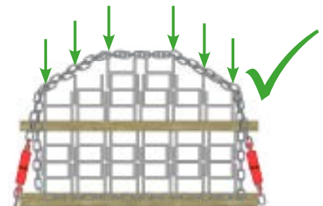
Pyramid load with intermediate timbers
