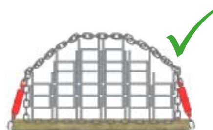
2 high tiers centre of load
