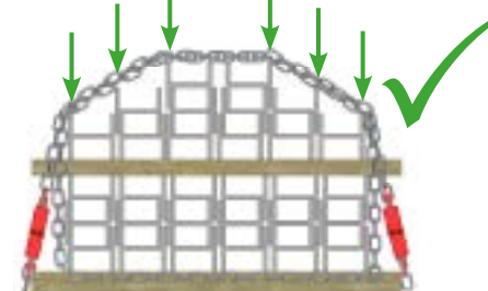
Pyramid load with intermediate timbers
